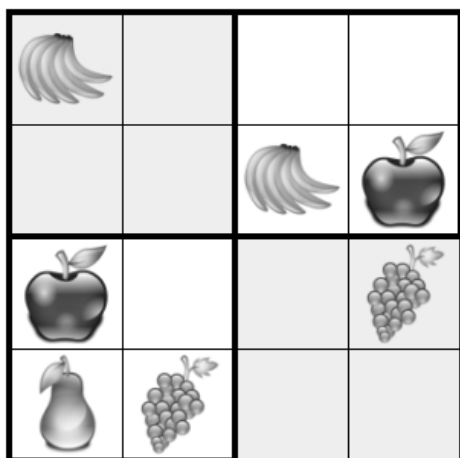
Sudoku 4x4, ID 134, Level 9
